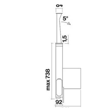
Side view, motor on the front
